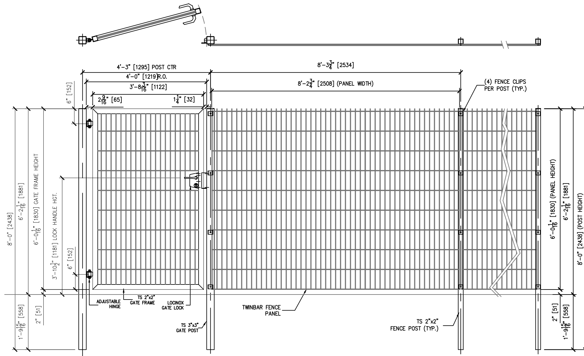
1 6'-0" HIGH TWINBAR FENCE w/ SINGLE SWING GATE TBFG SCALE: 1/2"=1'-0"
