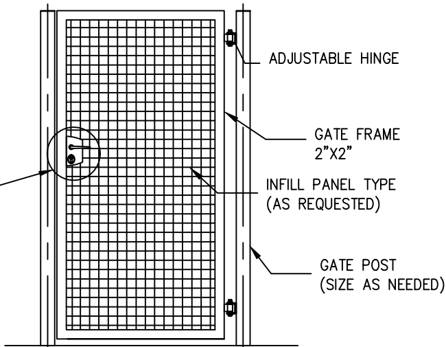
GATE LOCKING SET W/ HANDLE
