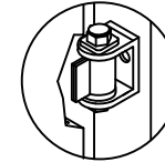
ADJUSTABLE GATE HINGE DETAIL
