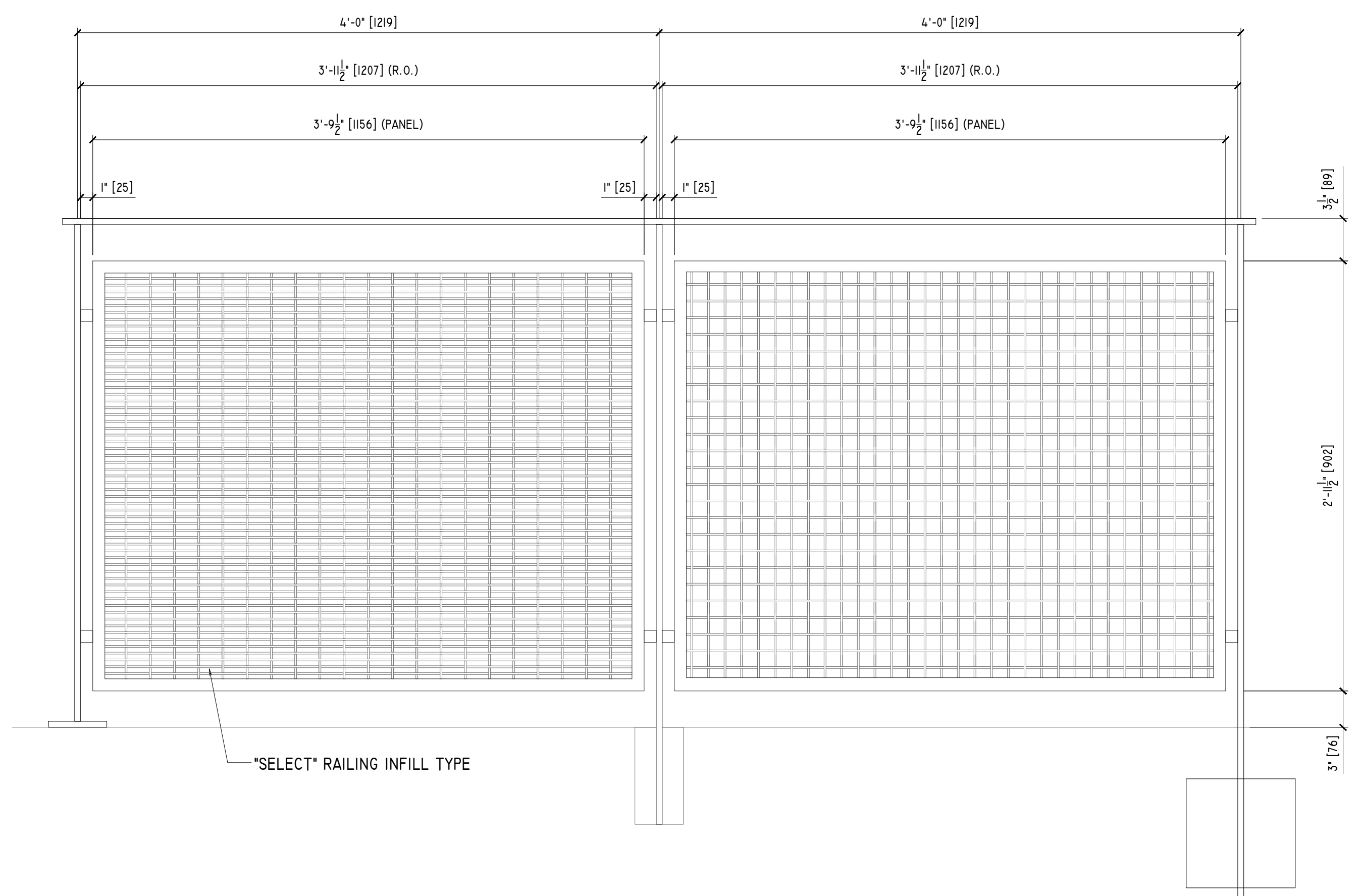
1 AI TYPICAL "SELECT" WOVEN MESH RAILING SYSTEM SCALE: 1"=1'-0"
