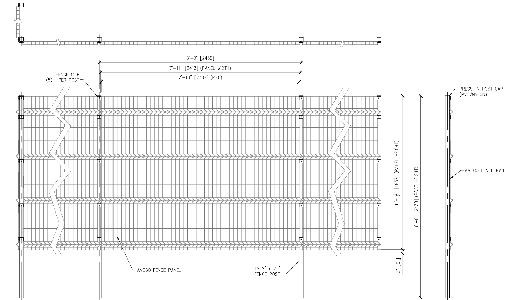
1 TYPICAL 6'-0" TALL AMEGO FENCE PARTIAL ELEVATION SK1 SCALE: 1/2"=1'-0"
