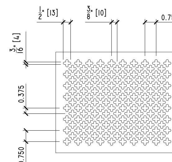
10 FULL CLOVERLEAF DECORATIVE AI SCALE: 3"=1'-0"
