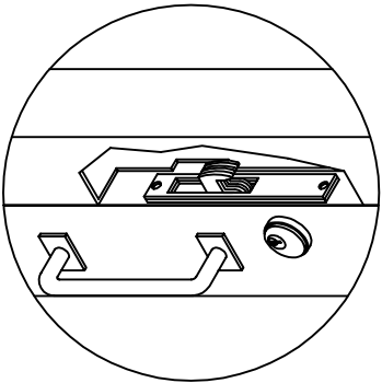
GATE LOCKING SET W/ HANDLE DETAIL
